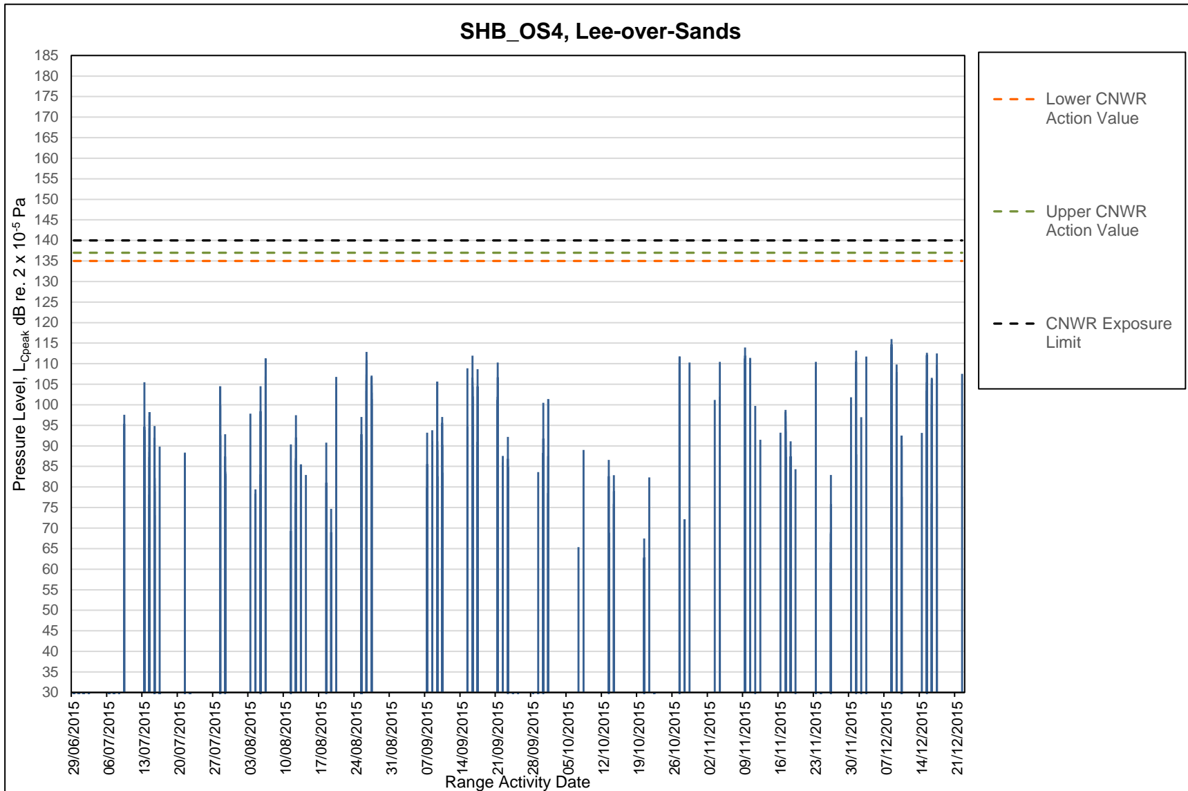
FIGURE A14: SUMMARY OF L CPEAK VALUES, SHB_OS4, LEE-OVER-SANDS, 28 TH JUNE 2015 – 31 ST DECEMBER 2015
